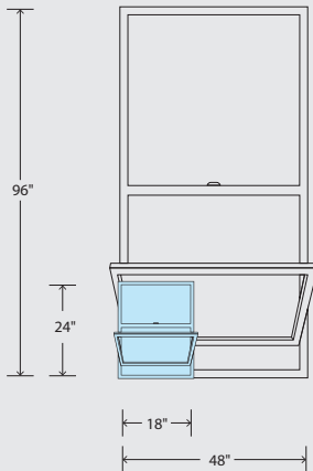
SINGLE- HUNG*
