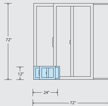
SINGLE-SLIDING
