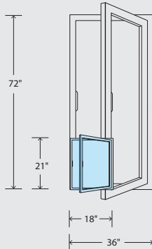
CASEMENT
