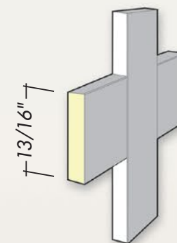
13/16 Inch Flat Grid
