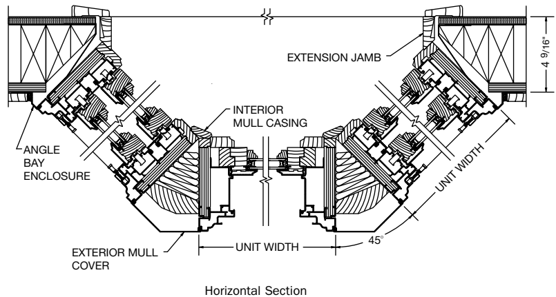
Horizontal Section
