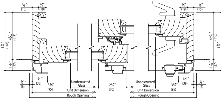
Horizontal Section
