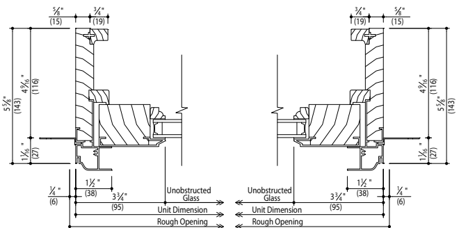
Horizontal Section
