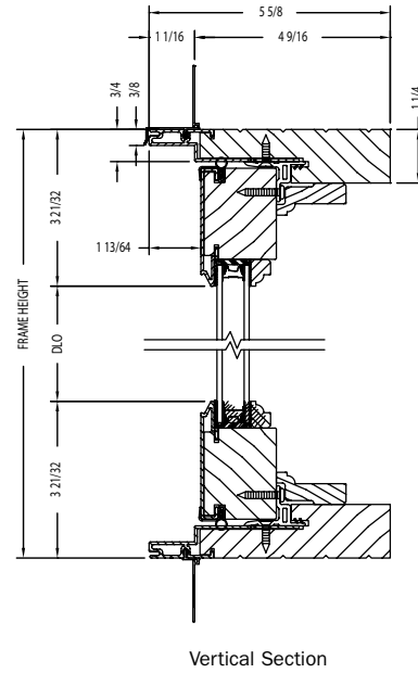
Vertical Section
