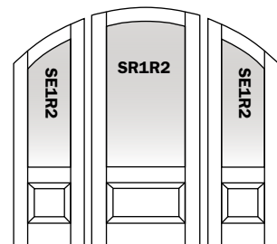
4 \frac{1}{16} " stiles, 4 \frac{1}{16} " top rail, 8" bottom rail & raised panel insert
