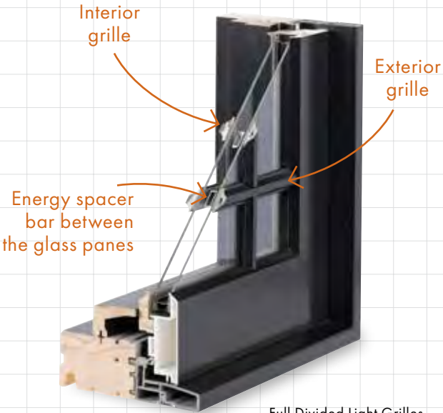
Full Divided Light Grilles with Energy Spacer Bar
