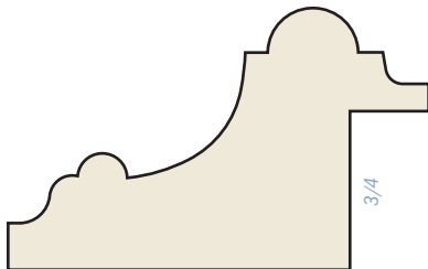
SM-64 Longwood Panel Mould 1-1/4 × 2 Poplar | SOLID PRIMED | POPPANSM64FPR
