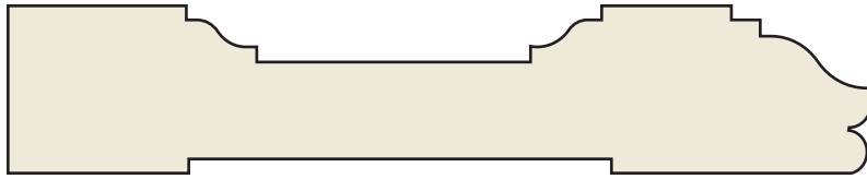
SM-83 13/16 × 4-1/8 Poplar | FINGER JOINTED PRIMED | POPCSM83FPR
