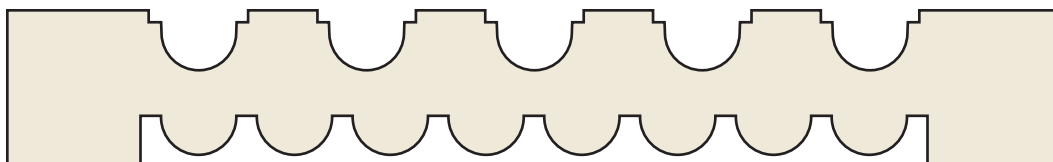
SM-85 Reversible Fluting/Reeding
