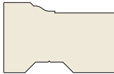
Brickmould #180 1-1/4 × 2 PVC | PVCWM18018
