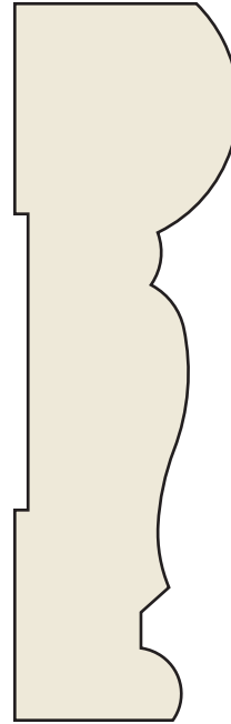
SM-49 Browning 1-1/16 \times 3-3/8 Poplar | FINGER JOINTED PRIMED | POPCHSM49FPR
