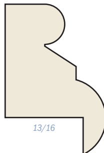
SM-60 Pine Picture Frame Mould 1-1/16 × 1-9/16 Poplar | FINGER JOINTED PRIMED | POPPANSM60FPR
