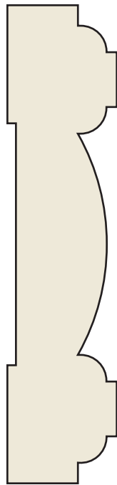
SM-79 Capitol Hill Casing 13/16 \times 3-1/2 Poplar | FINGER JOINTED PRIMED | POPCSM79FPR
