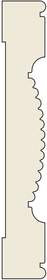
SM-80 Caroline Casing 3/4 × 5
