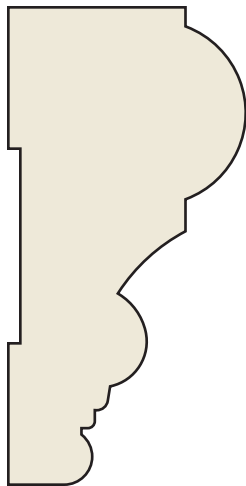
SM-43 Monfalcone 1-1/4 × 2-1/2 Poplar | FINGER JOINTED PRIMED | POPCSM43FPR
