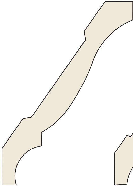
Crown #47 11/16 × 4-5/8 PVC | WM47PVC16
