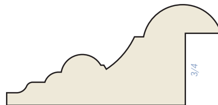
SM-143 Falcon Panel Mould 1-1/16 × 2-1/4
