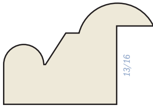
SM-60 Pine Picture Frame Mould 1-1/16 × 1-9/16 Poplar | FINGER JOINTED PRIMED | POPPANSM60FPR
