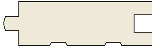
T&G 1 x 3 3/4 x 2-1/2 (2-1/4 Face) Red Oak | STAIN GRADE | 34ROAKFL
