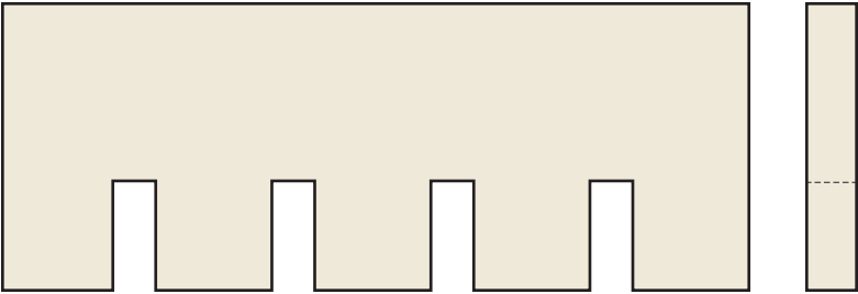
SM-33 Dentil 1/4 × 1-3/8 Pine | STAIN GRADE | SM33
