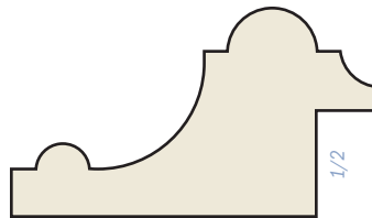
SM-62 Longwood Panel Mould 1 × 1-3/4
