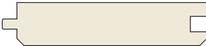
T&G 1 x 4 3/4 x 3-1/2 (3-1/4 Face) Mahogany | STAIN GRADE | PM14TG
