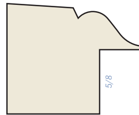
SM-68 Adams Backband 1-3/16 × 1-7/16 Pine | FINGER JOINTED PRIMED | SM68FPR Pine | STAIN GRADE | SM68
