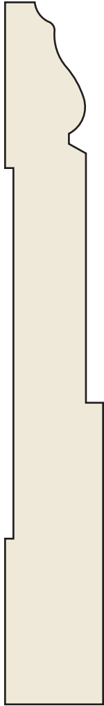
SM-266 Bates' Base 3/4 × 5-1/4
