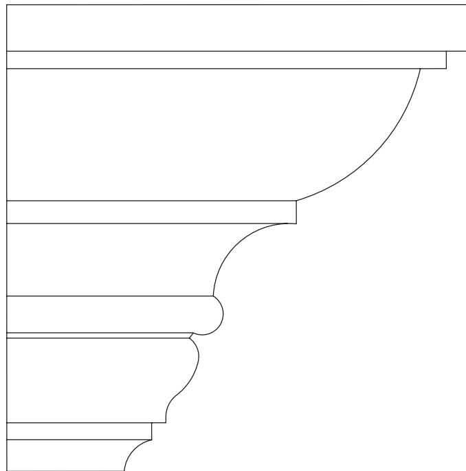
SM-712 Crown 13/16 × 4-1/2 Poplar | FINGER JOINTED PRIMED | POPCRSM712FPR
