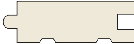
1 x 3 2-1/8 Face Yellow Pine | 34218SYPTGC
