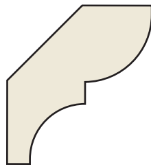
Bed Mould #75 9/16 × 1-5/8 PVC | WM75PVC16
