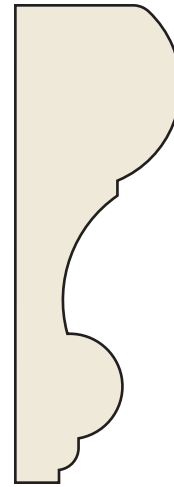
SM-45 Winston 7/8 × 2-1/2 Poplar | FINGER JOINTED PRIMED | POPCSM45FPR
