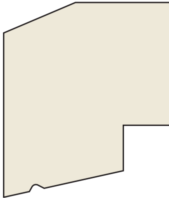
Historical Sill 1-3/4 × 2-1/32 PVC | MLD85310BP-16
