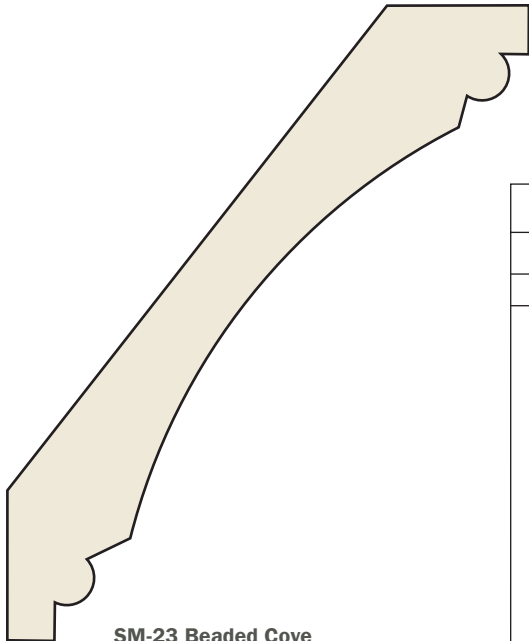
SM-23 Beaded Cove 13/16 × 4-1/4
