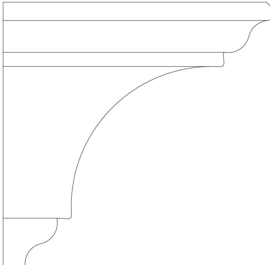
41M Crown 1-3/16 × 6-5/16 MDF | SOLID PRIMED | 41MDF16
