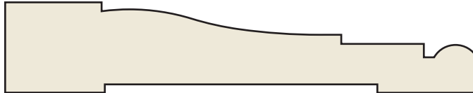
LWM-445 Beaded Casing 11/16 × 3-1/2 Pine | FINGER JOINTED PRIMED | LWM445P Pine | STAIN GRADE | LWM445S
