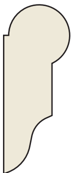
WM-276 Picture Mould 11/16 x 1-3/4 Pine | STAIN GRADE | WM276S
