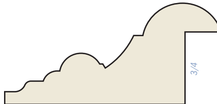
SM-143 Falcon Panel Mould 1-1/16 × 2-1/4 Poplar | FINGER JOINTED PRIMED | POPPANSM143FPR
