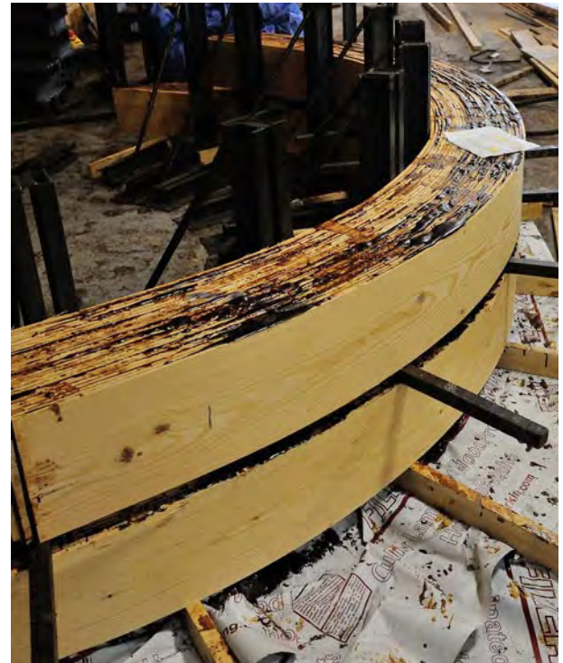
Clamping of Tight Radius Curve – ¾" Thick Laminations
