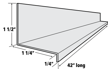
Aluminum Head Flash
