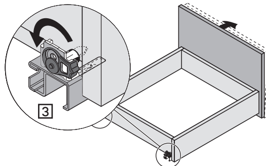
WHISPER TOUCH® FULL-EXTENSION UNDERMOUNT DRAWER RUNNER
