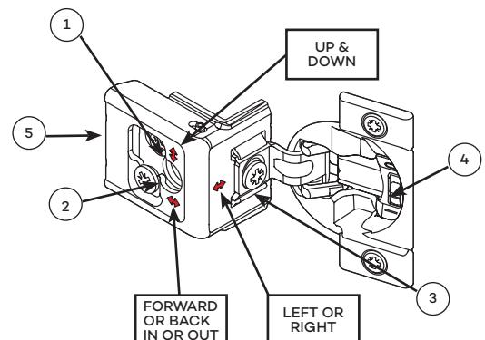
FULL OVERLAY
