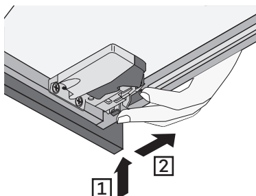
WHISPER TOUCH® FULL-EXTENSION UNDERMOUNT DRAWER RUNNER
