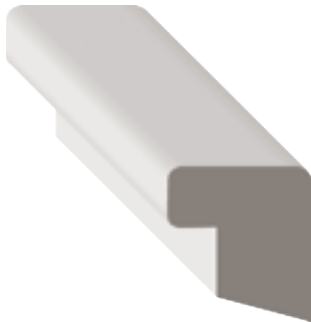
STOCK CODE 9701PRI (1522368) DIMENSIONS 3/4" x 1 3 / 16 " x 16' FITS 1/2" CASING 9705PRI (1522369) DIMENSIONS 3/4" x 1 1 / 16 " x 16' FITS 3/4" CASING PRI
