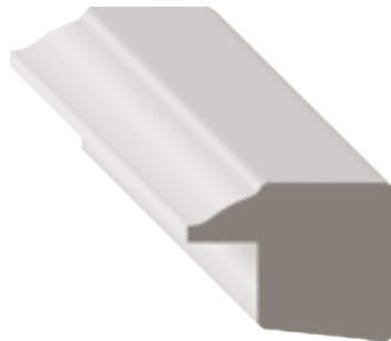
STOCK CODE 1016POP (1521170) DIMENSIONS 3/4" x 1" x RL FITS 1/2" CASING 1016POPI90 (1521171) DIMENSIONS 3/4" x 1" x 90" FITS 1/2" CASING POP
