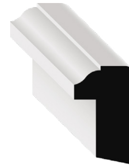
STOCK CODE 281LPRI (1521716) DIMENSIONS 1 1/16" x 1 1/8" x 16' FITS 1/16" TO 3/4" CASING
