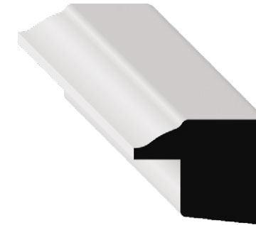
STOCK CODE 1016POP (1521170) DIMENSIONS 3/4" x 1" x 6-16' FITS 1/2" CASING
