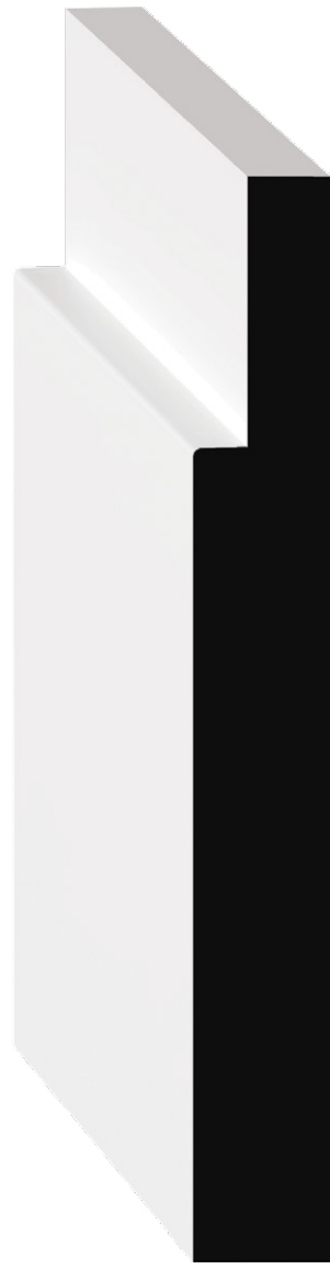
STOCK CODE 1683562 DIMENSIONS 5/8" x 5 1/4" x 16' MDF/UL
