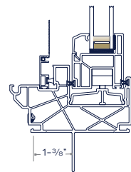
1 3/8" Mounting Fin Set-back
