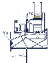
1 3/8" Mounting Fin Set-back w/ Stucco Key*
