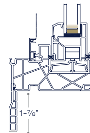
1 7/8" Contoured Flush Fin*
