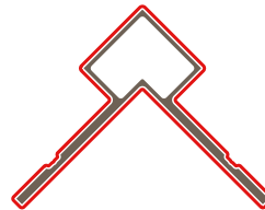
Outside Corner Trim UH60 (5-3/16" x 5-3/16")
