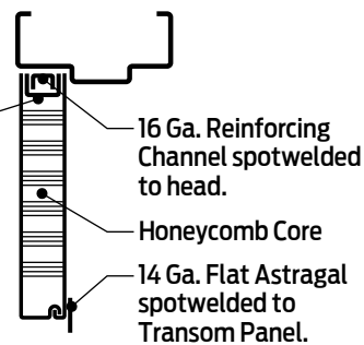
C TYPICAL LABEL SECTION
