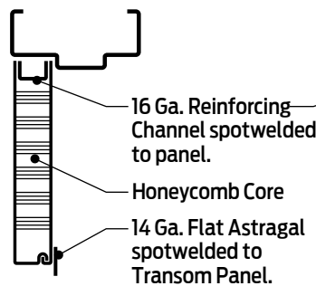
B TYPICAL NON-LABEL SECTION
