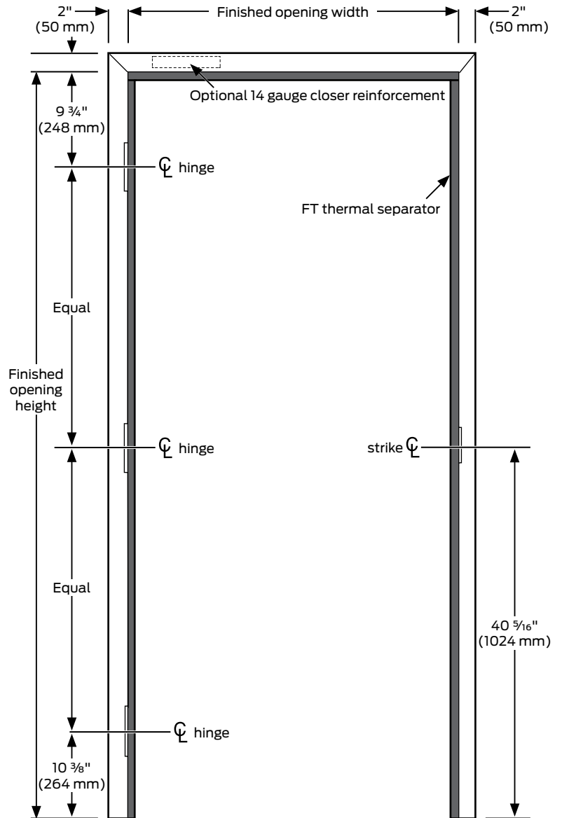
Figure 12.1: Elevation
