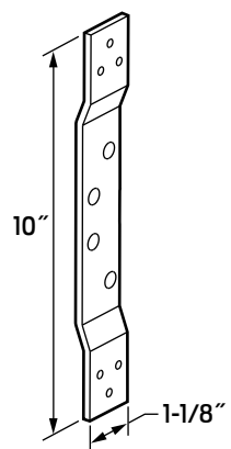
4" Hinge Detail Reinforcement .125" thick
