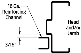
TYPICAL CHANNEL LOCATION
