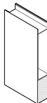
Optional 14 Gauge [0.067" (1.7 mm)] Closer Reinforcement
