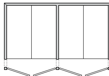
Double Door Applications
