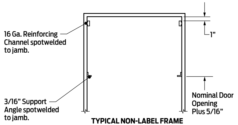
TYPICAL NON-LABEL FRAME
