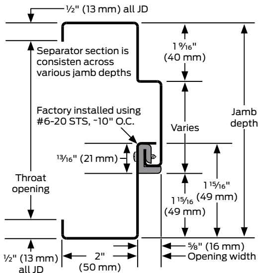
Figure 12.2: Standard double rabbet frame (factory assembled components)
