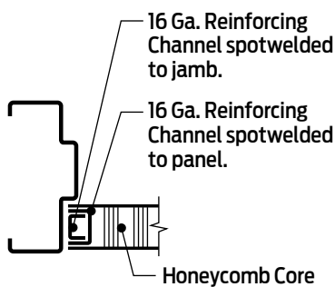
A TYPICAL JAMB SECTION
